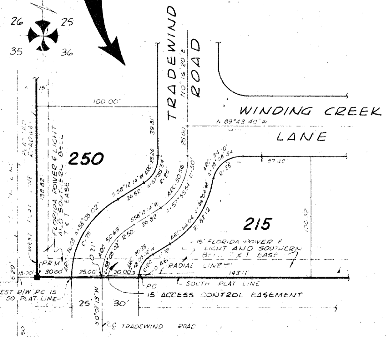
R/W DETAIL SCALE: 1"=30'
